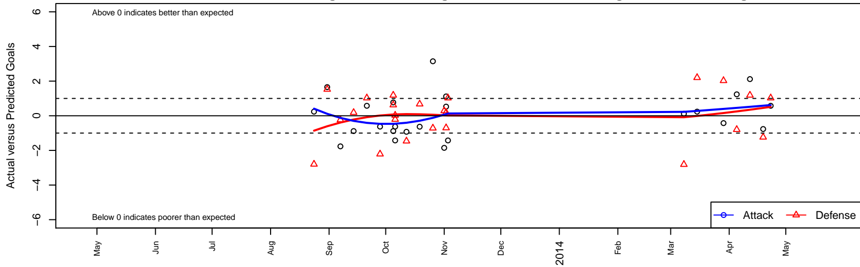
Boise Nationals Blue G02 Dots are actual minus expected GF (blue circles) and GA (red triangles). Blue line is smoothed change in attack strength. Red is smoothed change in defense strength.
